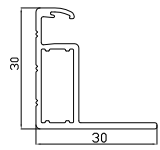
Section diagram of long frame profile
